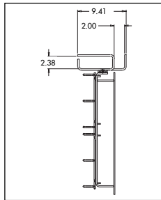
RIGHT: Side view of (left) 50M-900PD (right) 50M-900PLD
