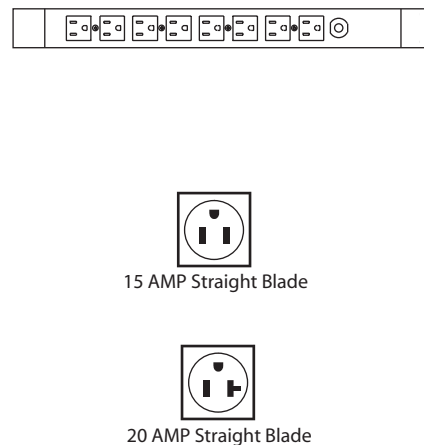
Receptacle Configurations
