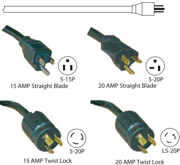
Plug Configurations
