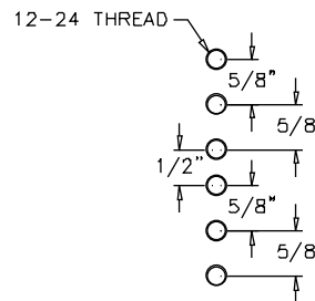
MOUNTING HOLE PATTERN
