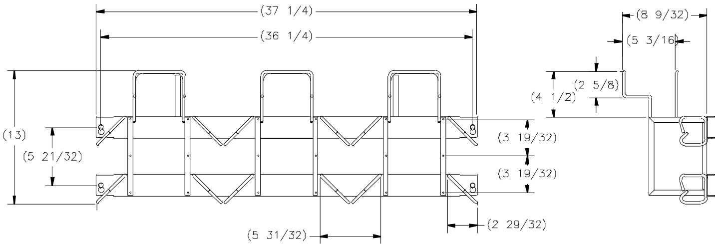
FRONT VIEW
