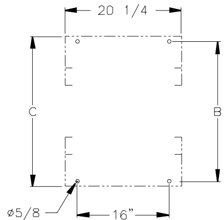
FOOT PRINT
