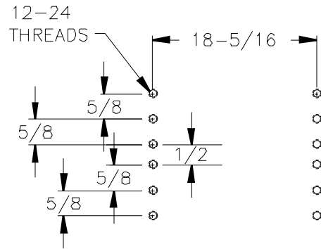
MOUNTING HOLE PATTERN
