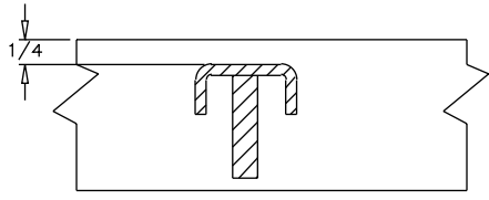
VIEW A-A REINFORCED
