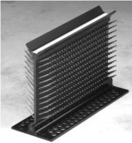
The 12 x 32 pin field configuration (above) provides the footprint for all AW Wire-Wrap Blocks.
