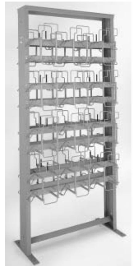
The double-sided 110D-7200 Frame* has modules on both sides to terminate 7,200 pairs.
