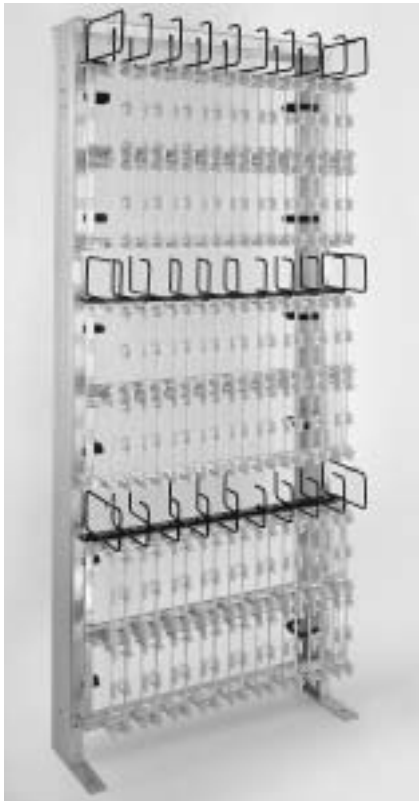
The 50M-2700LH Frame terminates 2,700 pairs and is equipped with H89 brackets already installed to save time at the job site.
