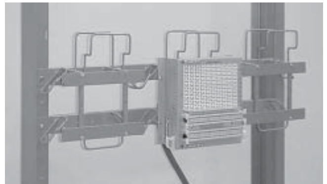
1880B1-100 mounted on 110D-900W using PAK-110D-188
