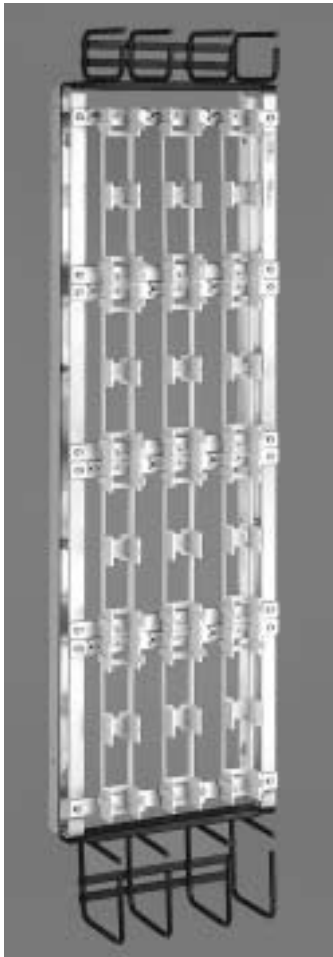
50M-600W terminates 600 pairs and can be used together with 50M-2000W.
