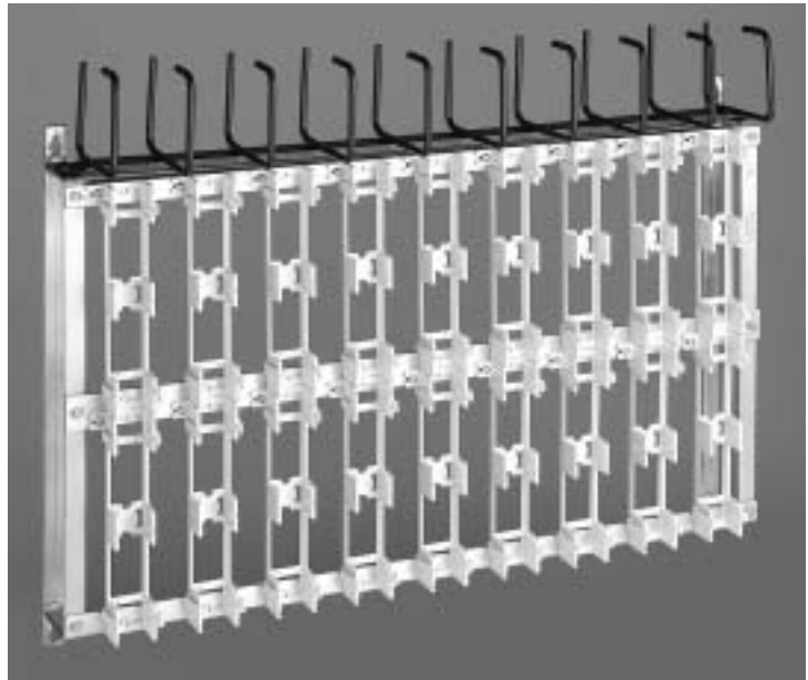
50M-900W terminates 900 pairs. It is the same module used on 50M frames but has been adapted to mount directly on the wall.
