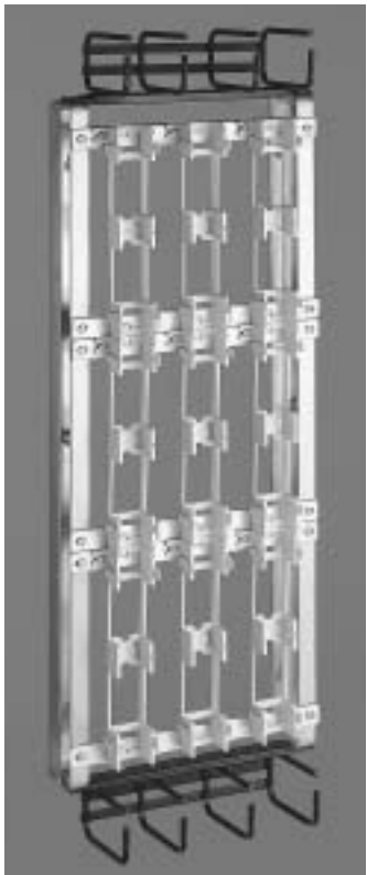
50M-450W terminates 450 pairs and can be used together with 50M-1500W.
