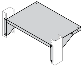
Shelf front flush to rack front
