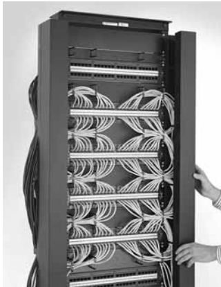
Vertical Organizer Covers (VO-84-T3CVL), left and (VO-84-T3CVR), right.
